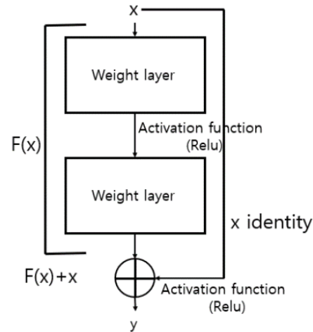
Figure 1. ResNet Process
