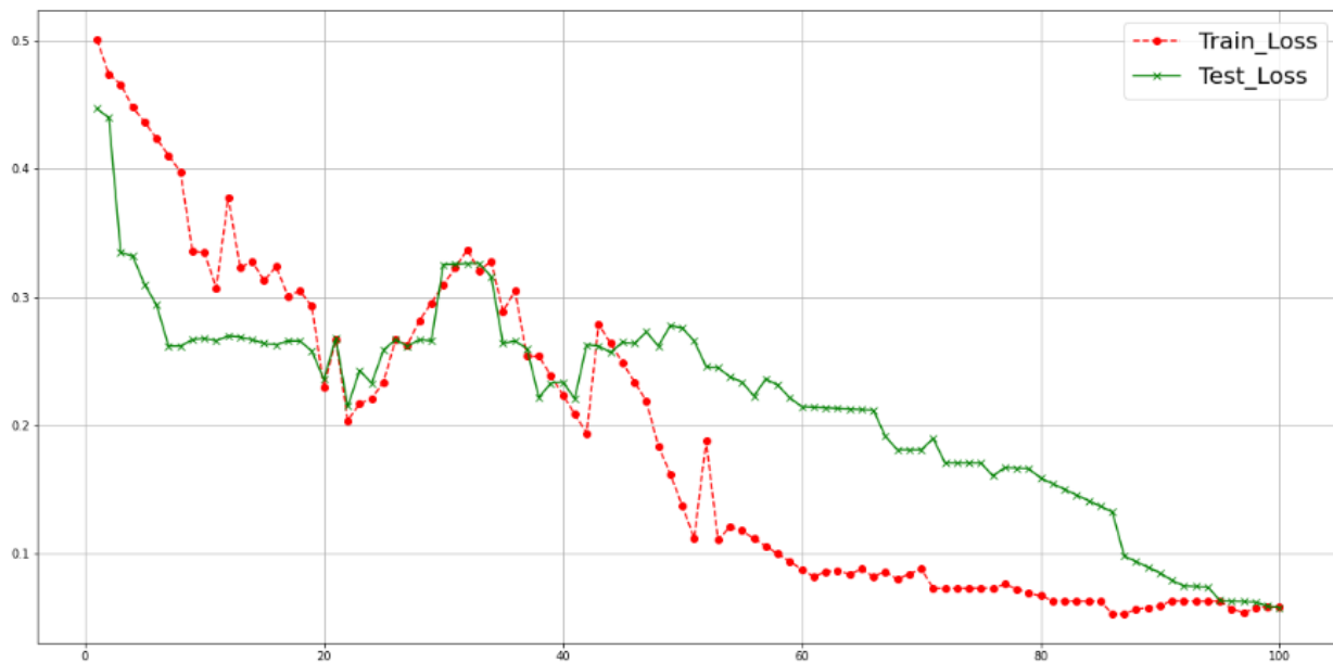
Figure 6. ResNet Loss (Training/Test).
